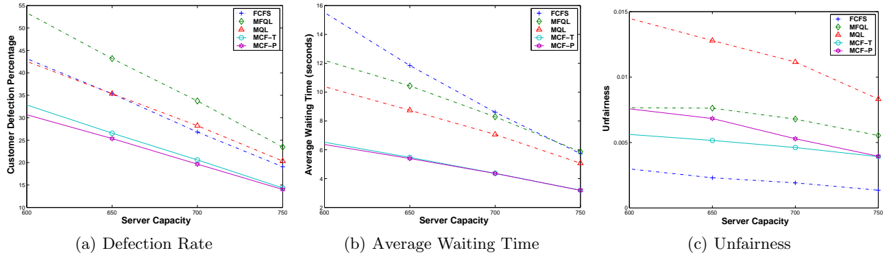
Figure 2: Comparisons among Various Scheduling Policies [ Transition Patching , \mu_{tol} = 0.5 minute]
