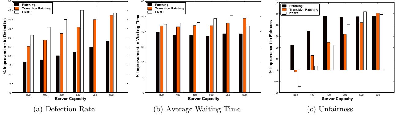
Figure 4: Percentage Improvements of MCF-P vs MQL [ \mu_{tol} = 0.5 minute]
