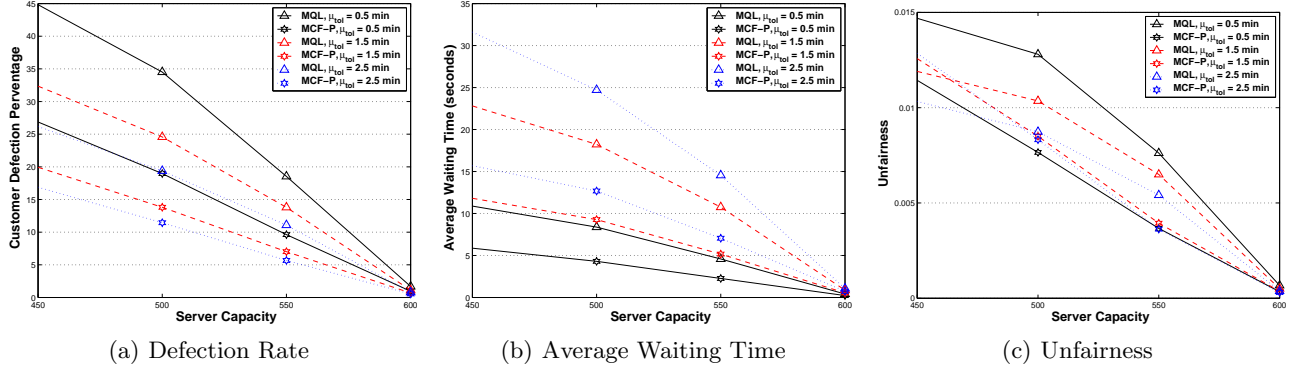
Figure 6: Comparisons between MQL and MCF-P under Variable Customer Waiting Tolerance [ ERMT ]
