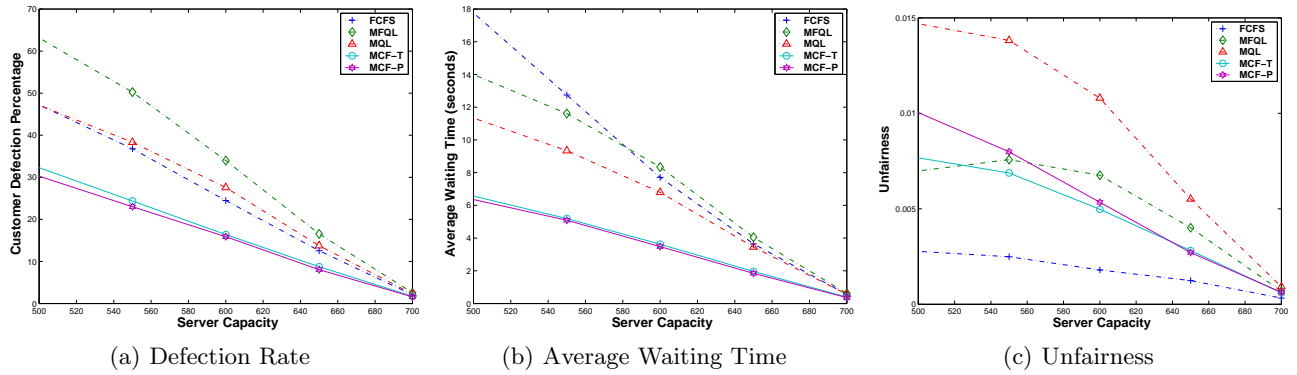
Figure 1: Comparisons among Various Scheduling Policies [ ERMT , \mu_{tol} = 0.5 minute]
