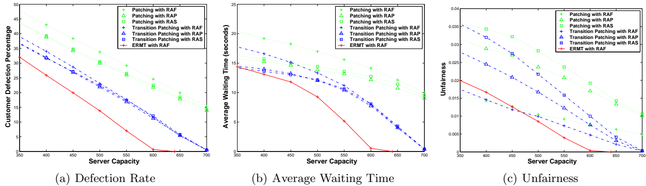
Figure 9: Comparisons among Stream Merging Techniques and MCF-P Variants [ \mu_{tol} = 1.5 minutes]
