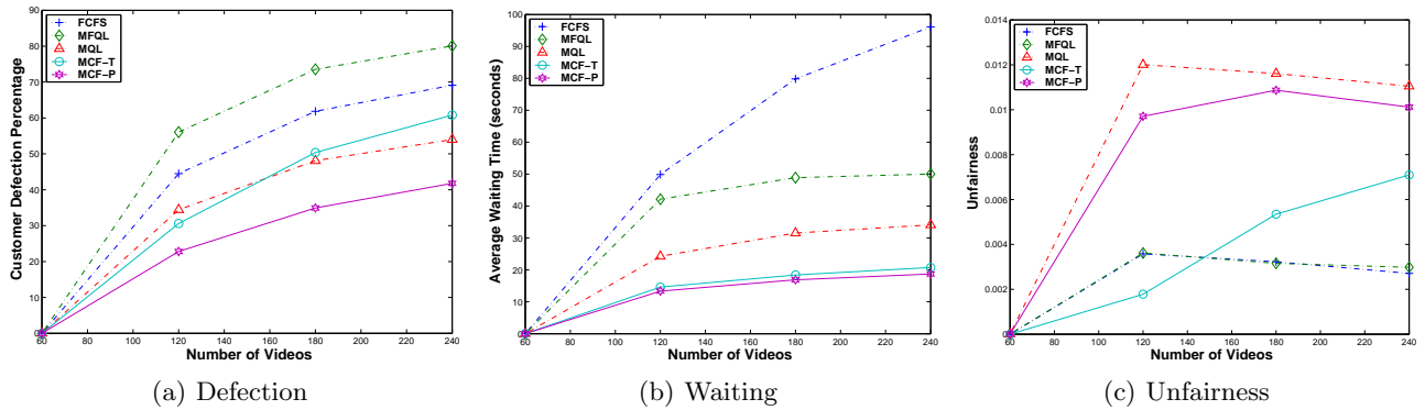
Figure 8: Impact of Number of Videos [ Transition Patching , 500 Server Channels, \mu_{tol} = 1.5 minute]
