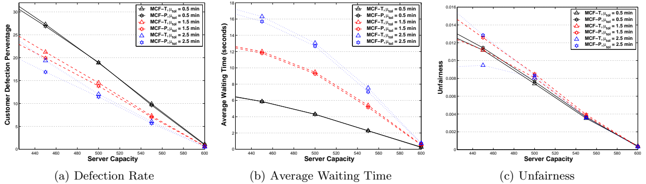
Figure 5: Comparisons between MCF-T and MCF-P under Variable Customer Waiting Tolerance [ ERMT ]
