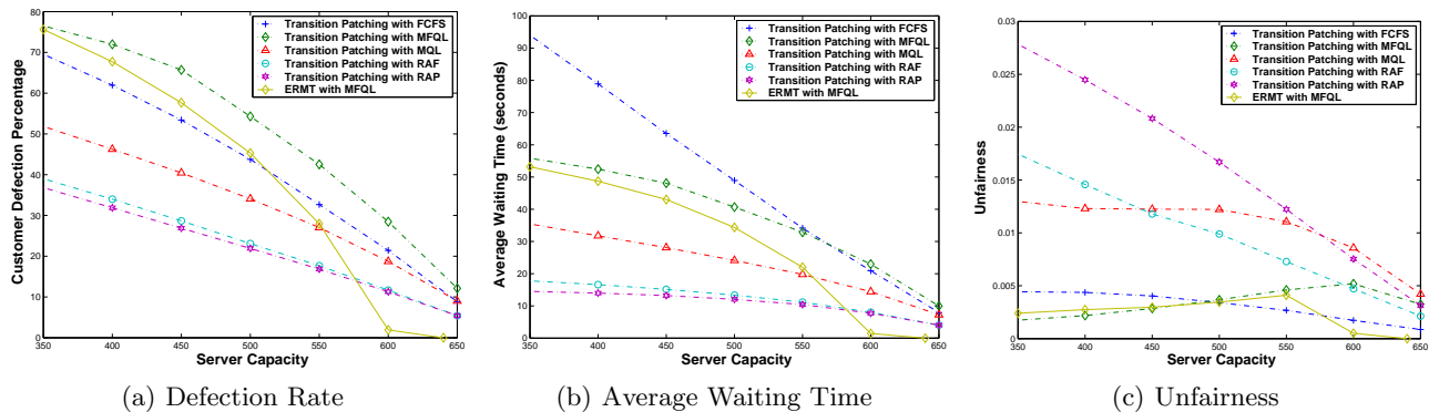
Figure 10: Comparing Stream Merging and Scheduling Performance [ \mu_{tol} = 1.5 minutes]
